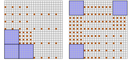
(a) Clustered; E = 0.80. (b) Scattered; E = 0.63.
