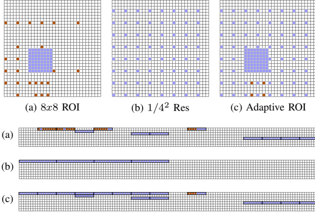
Fig. 4. Spatial and disk level layouts of ROI and reduced-resolution grids. The top row shows spatial grids with different write patterns. The lower grids show the element layout on disk. For disk-level storage, a block size of 8 is used for (a) and (c), and 16 for (b). Blue elements are primary elements; orange elements are secondary elements, or elements that are written as a by-product. Only primary and secondary elements are actually written to disk – blank elements are not written. (a) ROI write. Efficiency is 0.73. (b) Reduced-resolution write. Data on disk is not fragmented for reduced resolution writes, so efficiency is 1 irrespective of block size. (c) Adaptive ROI, combining ROI and reduced-resolution. Secondary elements for the ROI overlap with primary elements of the reduced-resolution write, so data is less fragmented, for efficiency of 0.97.
