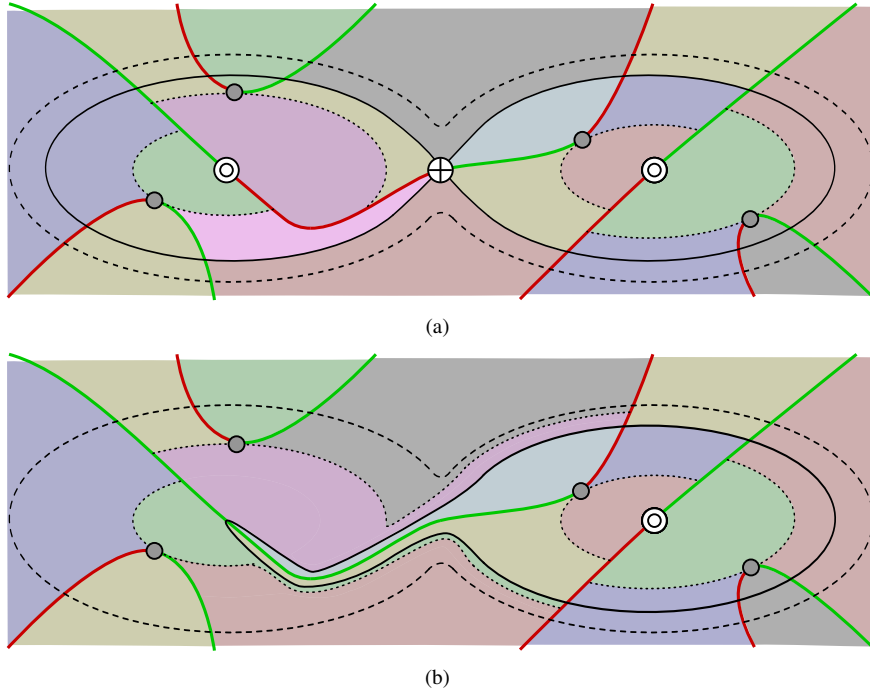
Figure 18: Effect of saddle cancellation on Jacobi segments and Jacobi regions. In addition to the level sets of BD points (dotted), level sets g^{-1}(g(\mathbf{s})) (solid) and g^{-1}(g(\mathbf{s}) - \epsilon) (dashed) are shown for reference. The Jacobi set is shown as a red-green curve, with color representing the criticality (i.e., restricted maximum or minimum). Jacobi regions corresponding to (a) the original Jacobi set \mathbb{J}(f, g) , and (b) the Jacobi set after cancellation, \mathbb{J}(f, g^*) , are shown in different colors.
