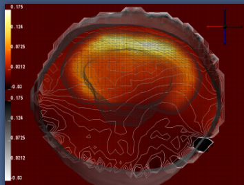
Visualization
