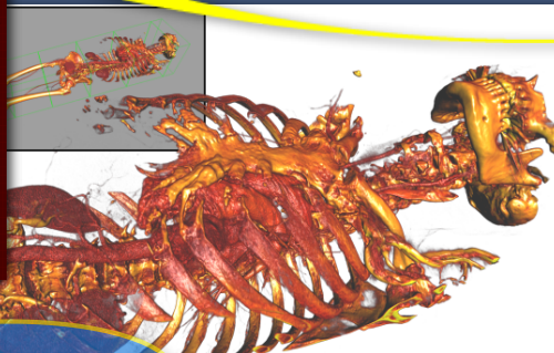
Visualization
