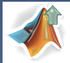
Matlab/Python
