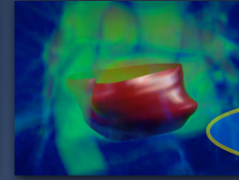
Image Processing
