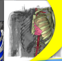
Geometry Processing
