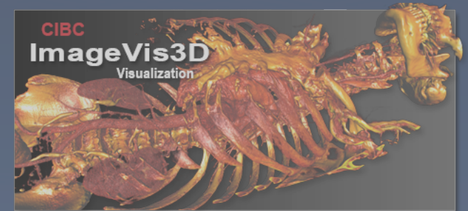
ImageVis3D (Visualization)
