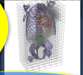
Geometry Processing
