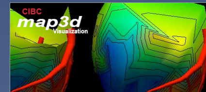
map3D (Visualization)
