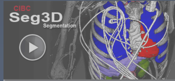
Seg3D (segmentation)
